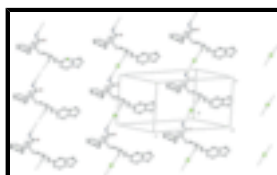
Fig. 2. Molecular packing of (I) viewed down the b axis; H-bonds are shown as dashed lines. For the sake of clarity, H atoms, not involved in hydrogen bonds, have been omitted.
